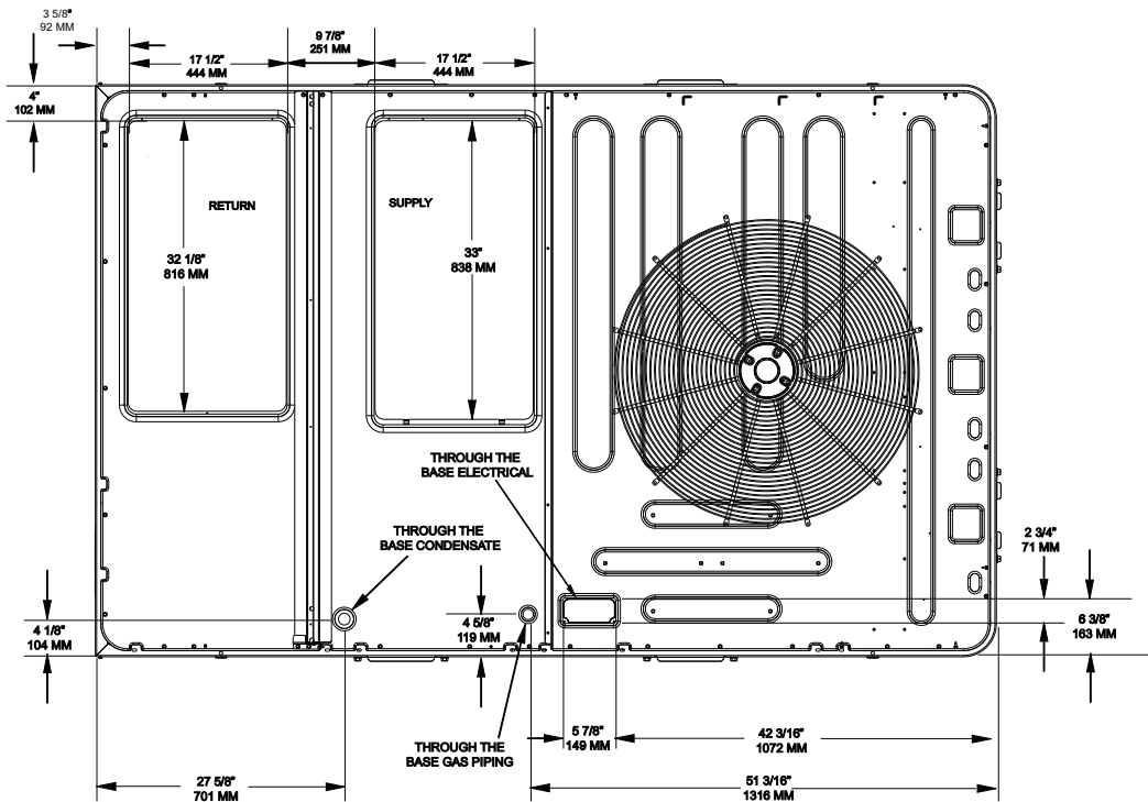
Figure 27. C.O cabinet – downflow airflow supply/return, through-the-base utilities
