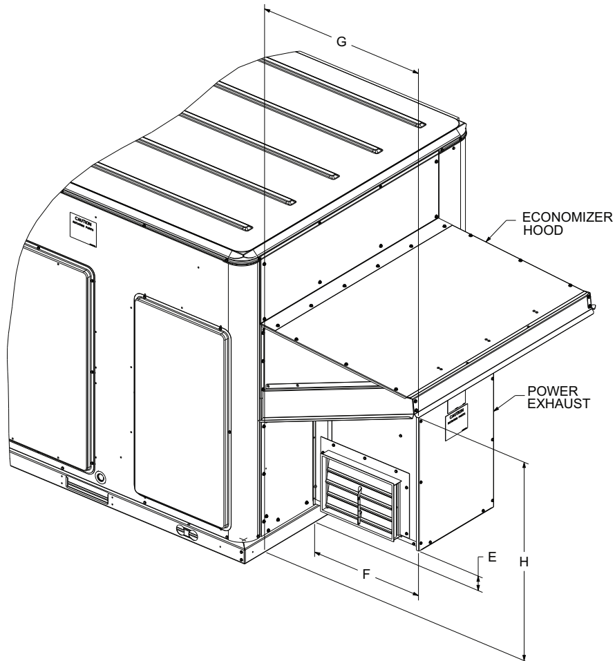
Figure 34. A.0, B.0, and C.0 cabinet – powered exhaust with low leak economizer
