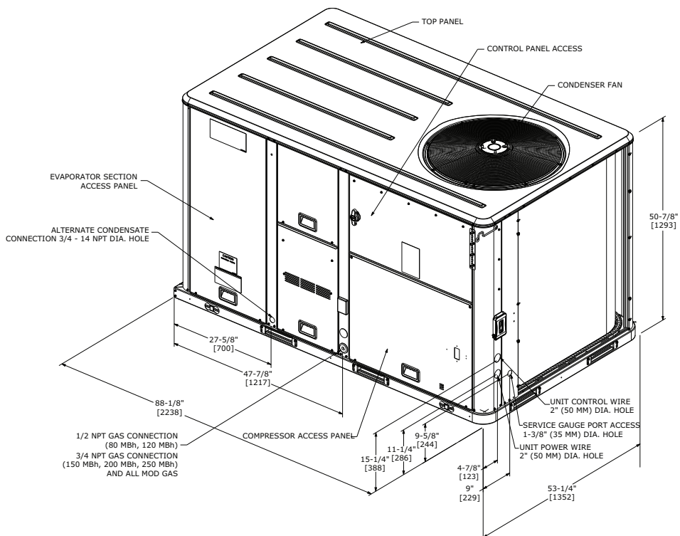
Figure 19. B.0 cabinet
